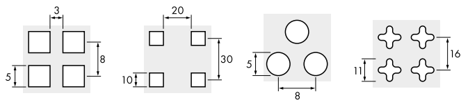
Blacha perforowana Qg 5-8
